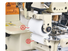
单向式后拖轮组(A表示齿轮, B表示平轮) Unidirectional rear drag wheel set (A for gear wheel, B for flat wheel)
