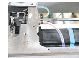
电机剪线结构 Motor wire cutting structure
